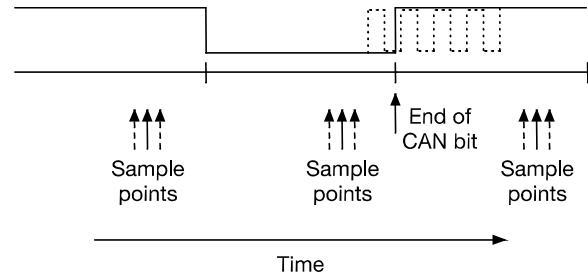
Figure 4: Out-of-band data in CAN
